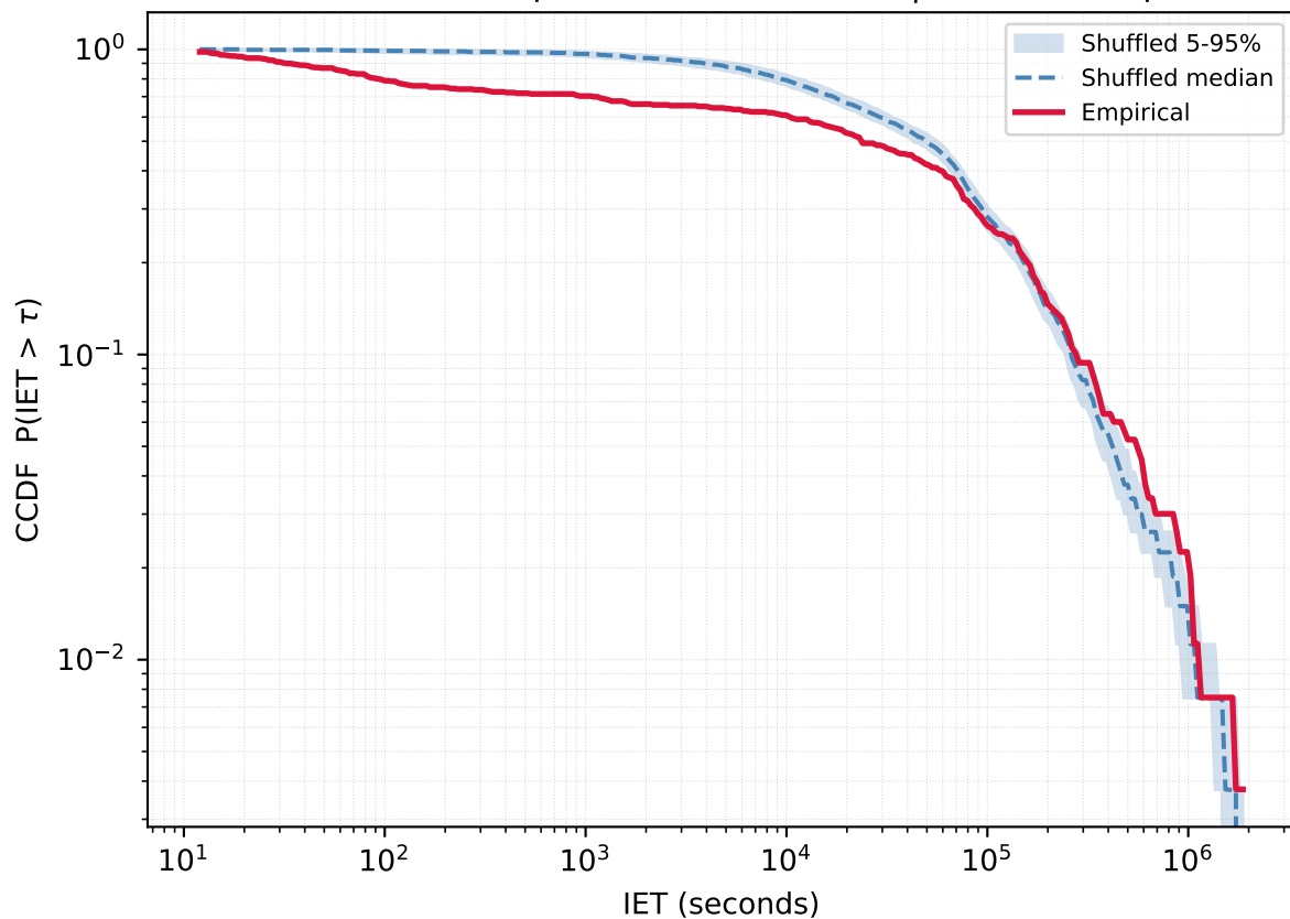
User 323949554 - Empirical vs Reshuffled | KS=0.282 p=0.000
